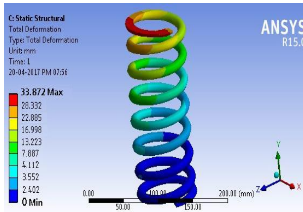
Figure.7: maximum deflection for hard drawn spring
