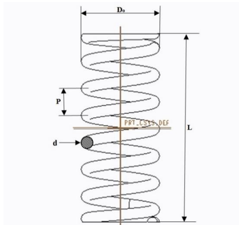
Figure.1: Design of helical spring
