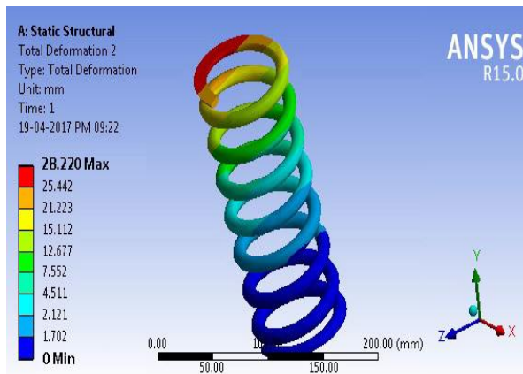
Figure.6: maximum deflection for chromesilicon spring
