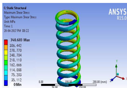
Figure.4: Maximum shear stress for Chrome silicon spring
