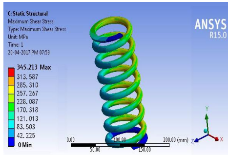
Figure.5: Maximum shear stress for harddrawn spring
