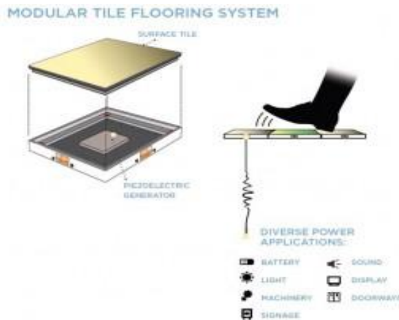
Fig 3: Piezoelectric tiles
