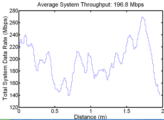
Figure 5 Average system throughput for FDMA user bandwidth allocation scheme
