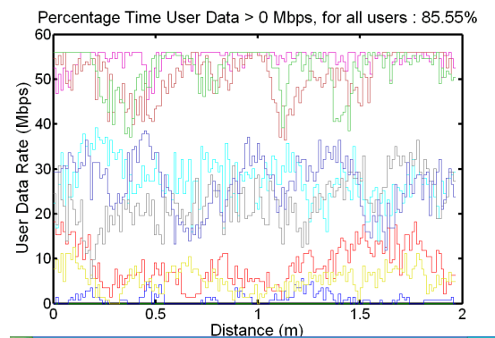
Figure 19 User data rate Variation for Random scheme
