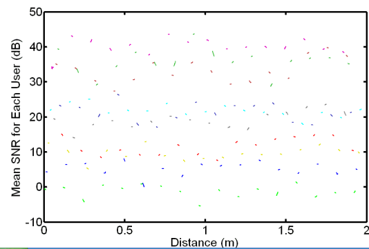
Figure 10 Mean SNR for individual user for TDMA user bandwidth allocation scheme
