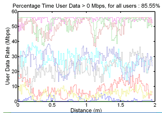
Figure 19 User data rate Variation for Random scheme
