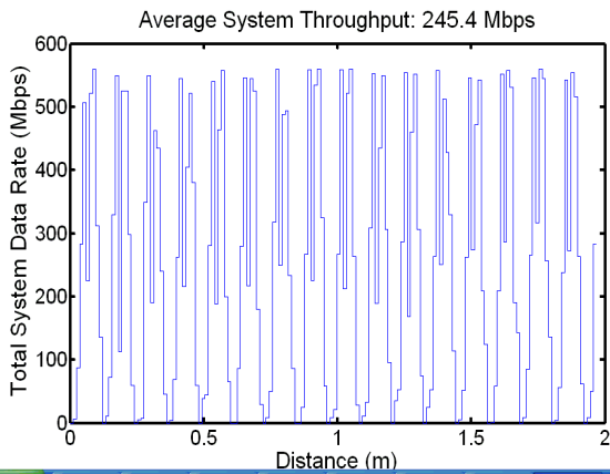
Figure 6 Average system throughput for TDMA user bandwidth allocation scheme
