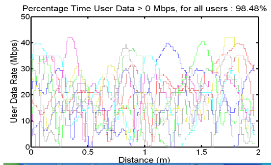
Figure 17 User data rate Variation for FDMA scheme
