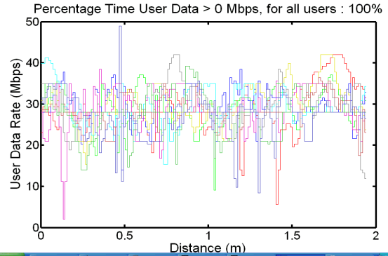
Figure 16 User data rate Variation for Adaptive MIMO-OFDM scheme
