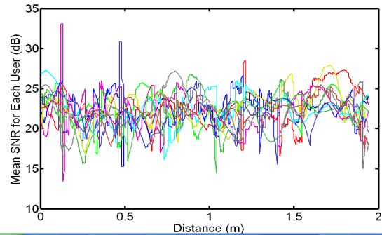
Figure 8 Mean SNR for individual user for Adaptive user bandwidth allocation MIMO-OFDM scheme
