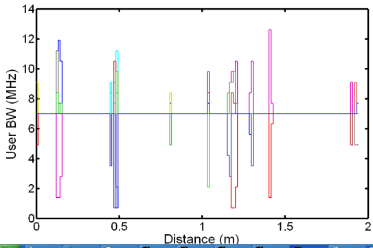
Figure 12 Adaptive User Bandwidth allocations
