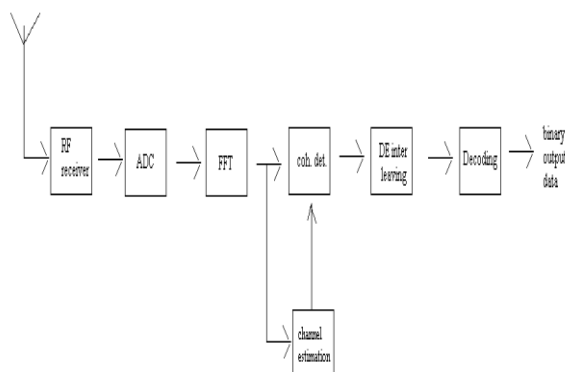
Figure 3 Block diagram of an OFDM receiver with coherent detection
