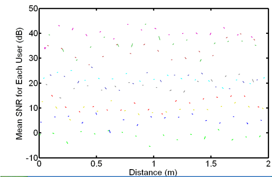
Figure 10 Mean SNR for individual user for TDMA user bandwidth allocation scheme
