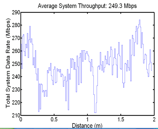
Figure 7 Average system throughput for Random user bandwidth allocation scheme
