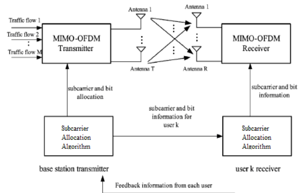
Figure 1 Bloch diagram of multiple antenna OFDM multicast system
