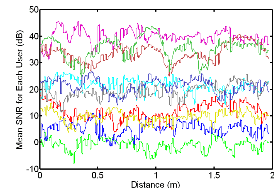
Figure 11 Mean SNR for individual user for random user bandwidth allocation scheme
