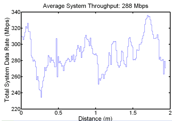
Figure 4 Average system throughput for Adaptive user bandwidth allocation MIMO-OFDM scheme
