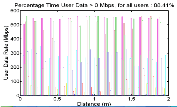
Figure 18 User data rate Variation for TDMA scheme
