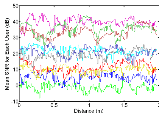
Figure 11 Mean SNR for individual user for random user bandwidth allocation scheme
