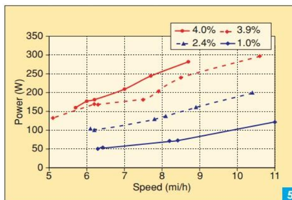
Fig.2 Influence of the slope of the power versus speed curve
