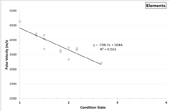
Fig 19: V-meter results versus condition state of elements
