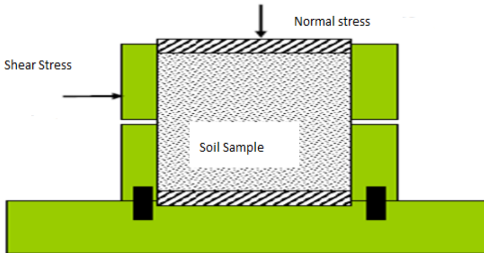
Figure 1: Test Apparatus
