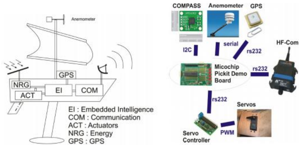
Fig. 1 Hardware Architecture
