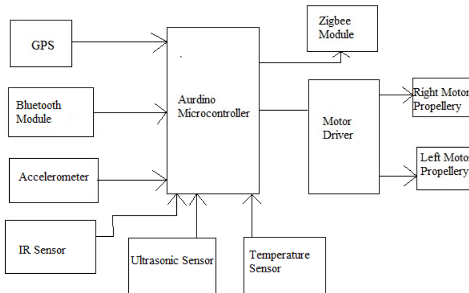
Fig. 2 Block Diagram
