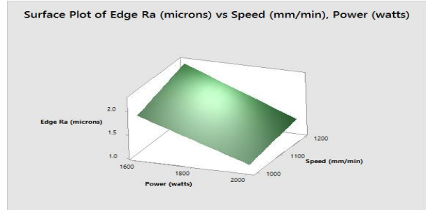
Fig. 7 Surface plots for Edge Ra (microns)
