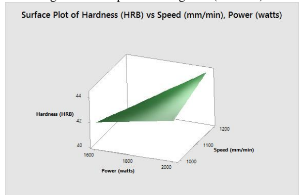
Fig. 8 Surface plots for Hardness (HRB)
