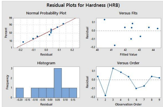
Fig. 5. Residual plots for Hardness (HRB)
