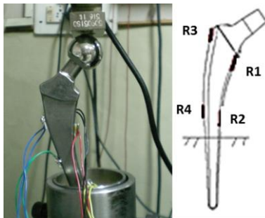
Fig.1 Position of LVDTs for construct A
