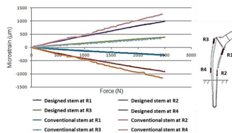
Fig. 4 Micro-strain vs. Force for newly designed and conventional stems
