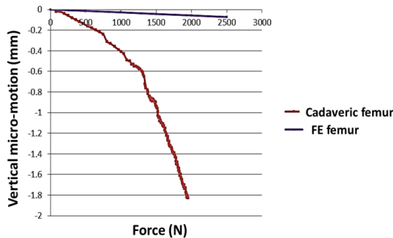
Fig.7 Micromotion vs. Force for the stem-dry cadaver femur construct with experimental and FE values superimposed
