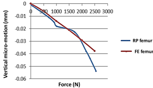
Fig.6 Micromotion vs. Force for the stem-SLS femur construct with experimental and FE values superimposed
