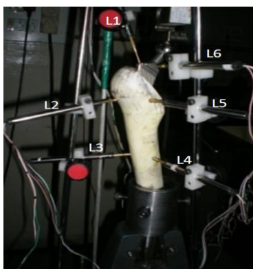
Fig. 2b Construct B (RP femur)
