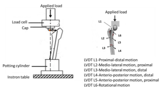
Fig. 2a. Position of LVDTs for constructs B and C
