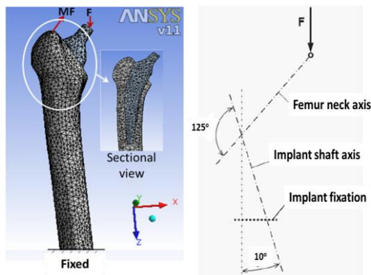
Fig. 3 Loading condition for the FE models
