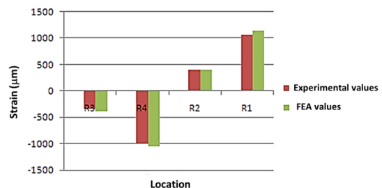
Fig. 5 Comparison of experimental and FEA values of strain at different locations along the stem
