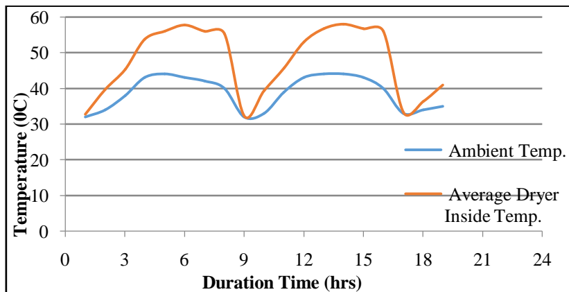
Figure VIII Graph showing Duration (Drying) Time vs Temperature
