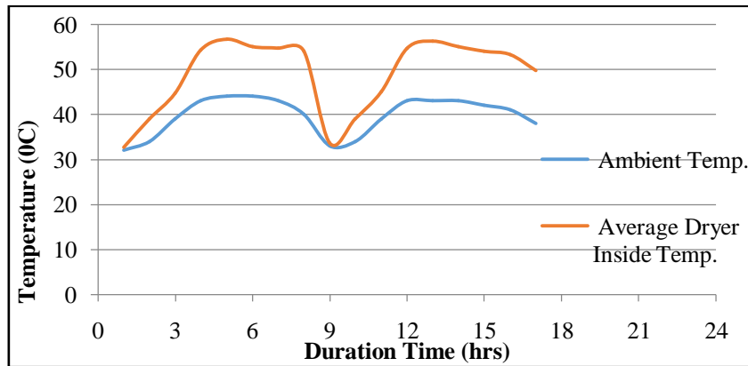
Figure IX Graph showing Duration (Drying) Time vs Temperature
