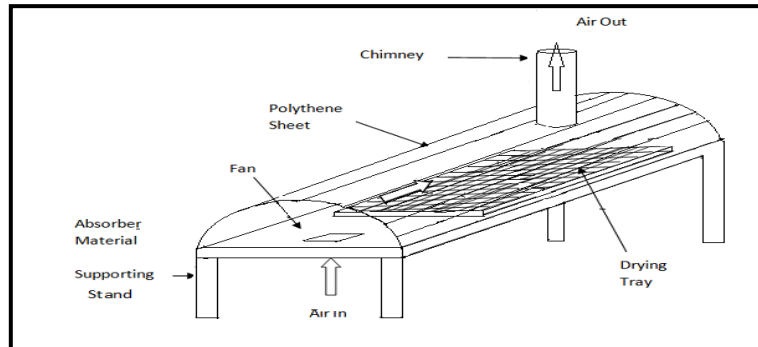
Figure I Schematic of Solar Tunnel Dryer
