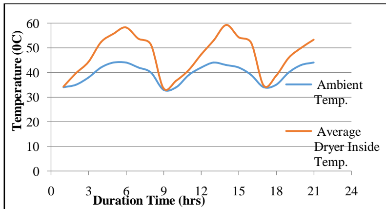
Figure VII Graph showing Duration (Drying) Time vs Temperature
