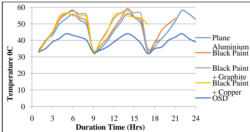
Figure X Graph showing Duration (Drying) Time vs Temperature
