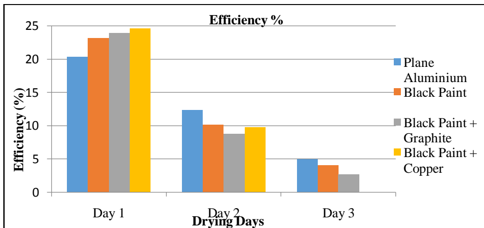
Figure XI Graph showing per Day efficiency of Solar Tunnel Dryer
