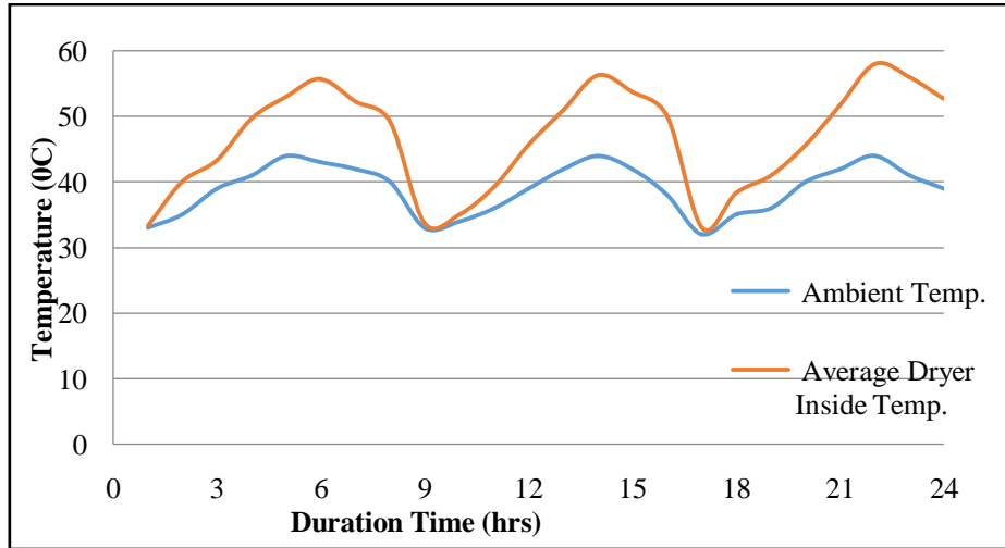
Figure VI Graph showing Duration (Drying) Time vs Temperature
