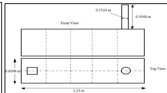
Figure III Front View and Top View of Dryer
