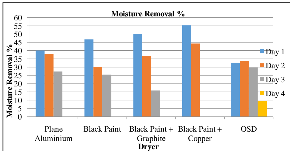
Figure XII Graph showing Per Day Moisture Removal
