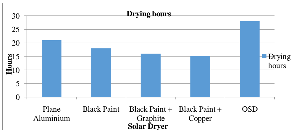
Figure XIII Graph showing Variation in Drying hours for Dryer
