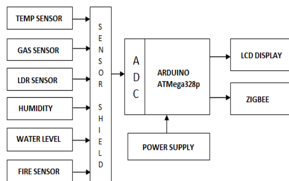
Fig. 1. Block diagram of Tx
