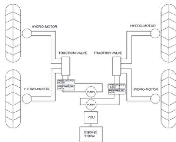
Fig.1. layout of hydrostatic power transmission system
