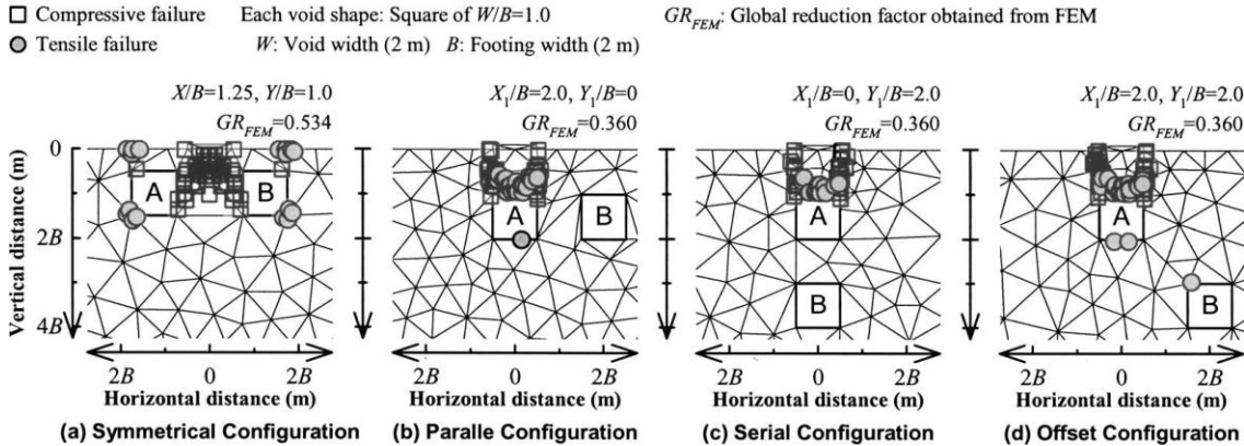
Fig. 8: Failure zones at yielding pressure ( q_y ) for various configurations [8]
