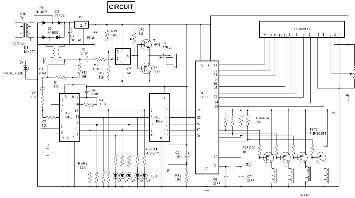
Figure 1.b: Circuit diagram of receiver
