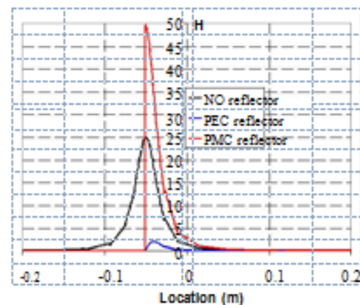
Fig.1 Magnetic field distribution versus distance from the loop source, calculated with COMSOL. Note that for an ideal PMC, the magnetic field is zero on the far side of the coil
