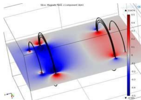
Magnetic field distribution of the WPT system when D=8\text{ cm} and f=25\text{ MHz}
