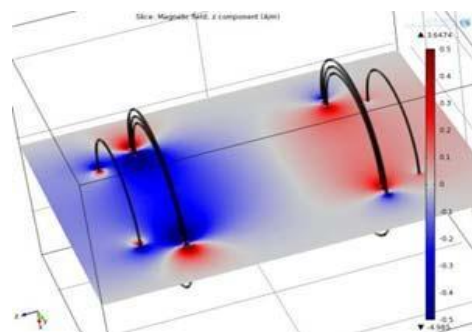
Magnetic field distribution of the WPT system when D=8 cm and f=25 MHz
