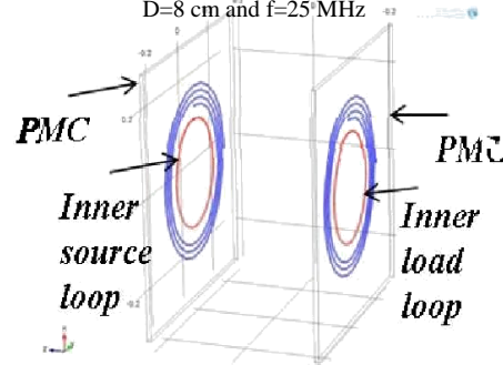
Fig.3 Geometry of the WPT system with PMC reflectors on both sides.
