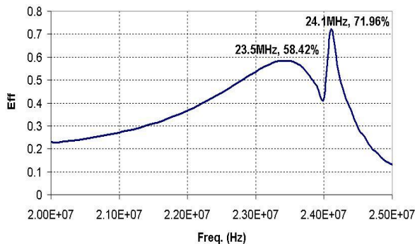
Fig.4 Power transfer efficiency of the WPT system with PMC as reflectors
