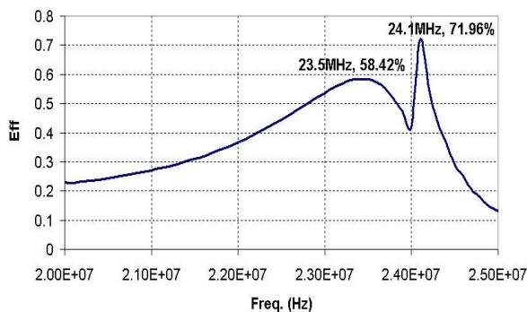
Fig.4 Power transfer efficiency of the WPT system with PMC as reflectors
