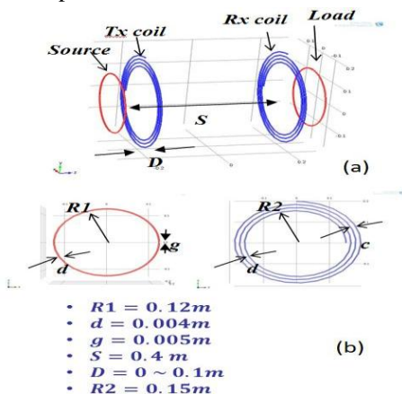
Fig. 2 (a) The resonant coupling based WPT system used in numerical studies; (b) Geometry of non-resonant loop and resonant coil in the WPT system, and corresponding parameters.
