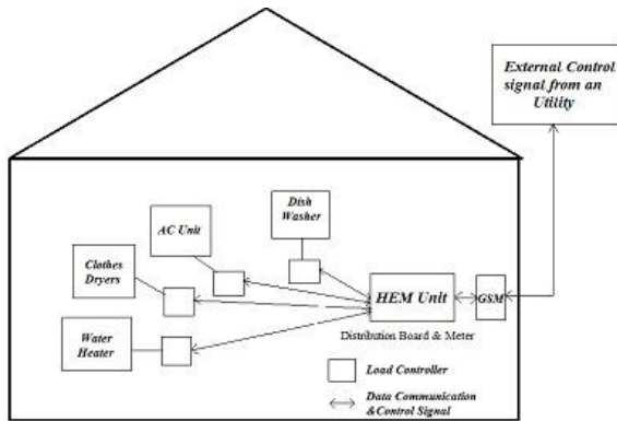
Fig 1. HEM architecture
