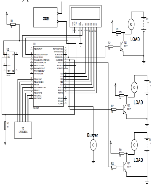
Fig 3.Circuit Diagram for Proposed System
