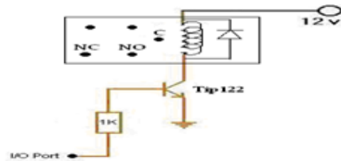
Fig 2. Relay Circuit
